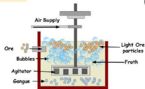
Froth Flotation Process
